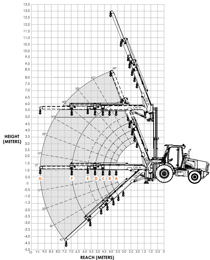
LOAD CHART
