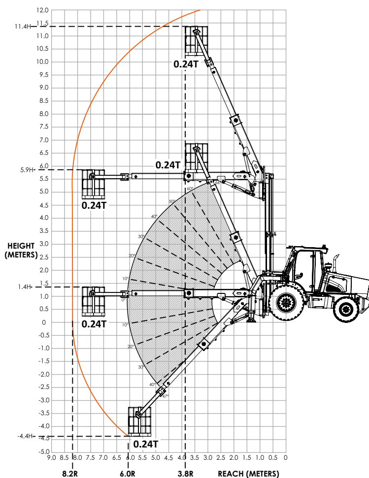
LOAD CHART
